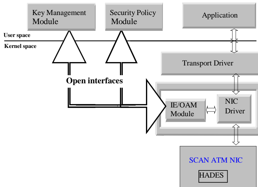
Figure 3 The software modules architecture
